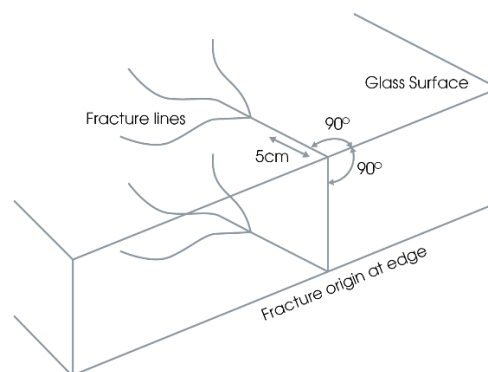
Diagram 4. High stress thermal breakage
