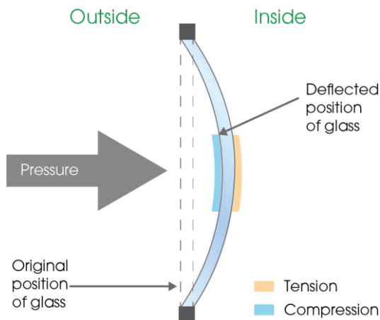
Diagram 1. Deflection: tension and compression
